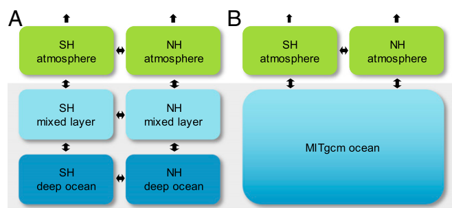
Fig. 1. Schematic diagrams showing the box model (A) and the MITgcm setup (B). The box model has three layers that represent the atmosphere, ocean mixed layer, and deep ocean. Each layer has two boxes that indicate the NH and the SH. The MITgcm setup replaces the four ocean boxes with the MITgcm ocean but keeps the atmospheric boxes unchanged. One-way arrows indicate CFC-11 atmospheric loss; two-way arrows indicate CFC-11 transport into/out of the box.
